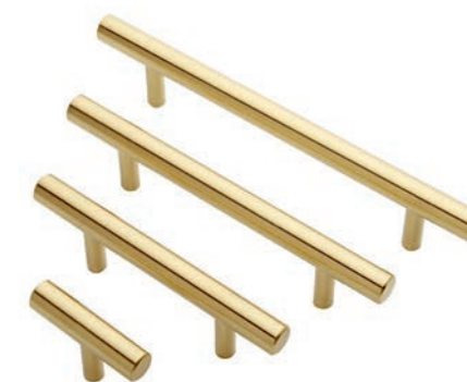
MH-79-1 Brass L150mm H35mm Ø12mm CC96mm Brass color
